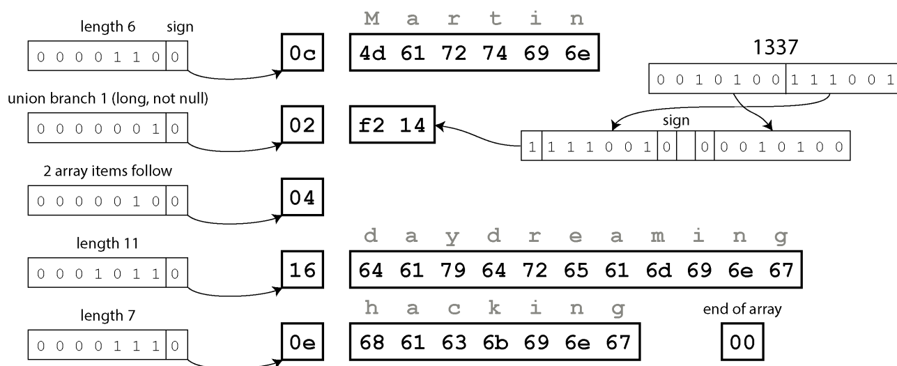
Figure 5-4. Our record encoded using Avro
